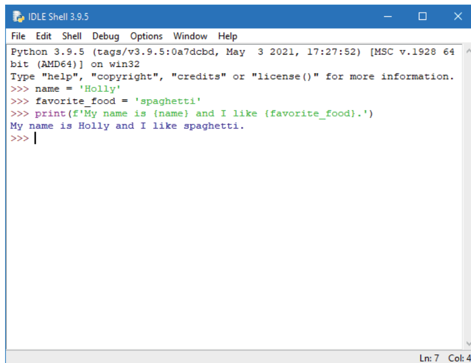
Figure B-2 The figure illustrates a IDLE shell window.
