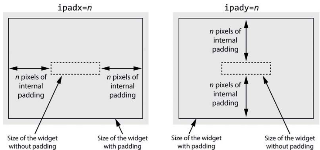
Figure 13-13 Horizontal and vertical internal padding
